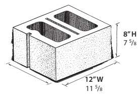
12" CORNER / SASH UNIT WT: 43.0 LBS.
