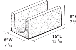
8" SOLID BOND BEAM UNIT WT: 43.5 LBS.
