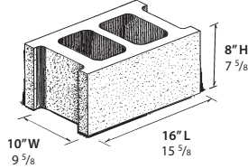
8" STRETCHER UNIT WT: 36.25 LBS.
