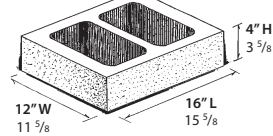
12" PILASTER UNIT WT: 25.5 LBS.
