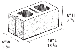
6" CORNER / SASH UNIT WT: 29.0 LBS.
