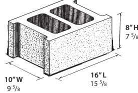
10" STRETCHER UNIT WT: 39.5 LBS.
