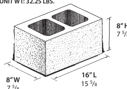
8" PILASTER UNIT WT: 32.25 LBS.
