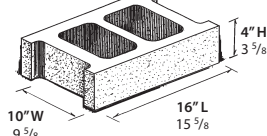
8" STRETCHER UNIT WT: 16.25 LBS.
