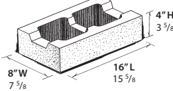
8" RESTRICTED BOTTOM BOND BEAM UNIT WT: 16.25 LBS.
