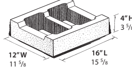
12" RESTRICTED BOTTOM BOND BEAM UNIT WT: 22.5 LBS.
