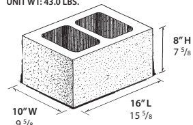
10" PILASTER UNIT WT: 43.0 LBS.
