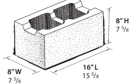
8" RESTRICTED BOTTOM BOND BEAM UNIT WT: 36.25 LBS.
