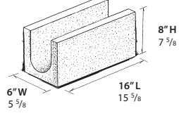
6" SOLID BOND BEAM UNIT WT: 32.25 LBS.
