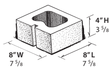
8" HALF UNIT/SASH UNIT WT: 10.4 LBS.
