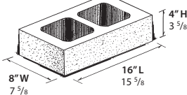
8" PILASTER UNIT WT: 16.25 LBS.
