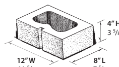
12" HALF UNIT/SASH UNIT WT: 13.0 LBS.
