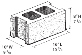
6" STRETCHER UNIT WT: 29.0 LBS.
