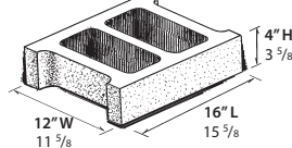
12" STRETCHER UNIT WT: 25.5 LBS.
