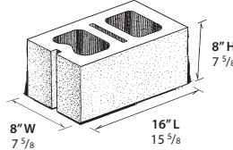
8" CORNER / SASH UNIT WT: 36.25 LBS.
