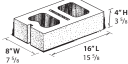
8" CORNER / SASH UNIT WT: 16.25 LBS.
